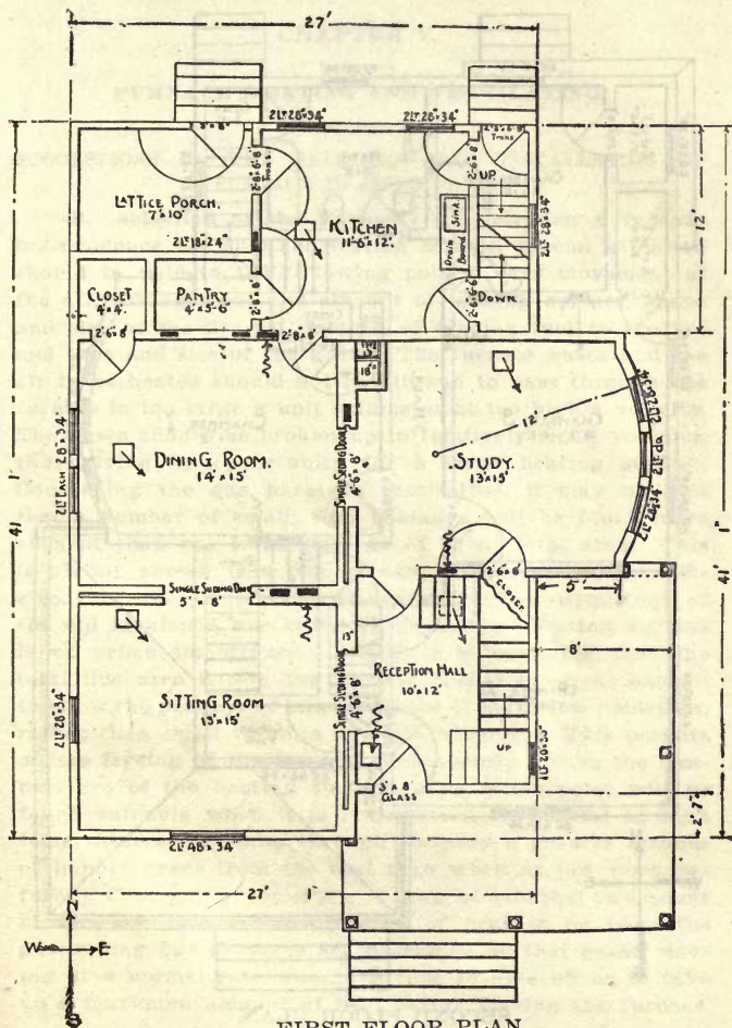
FIRST FLOOR PLAN, Ceiling 10'.
